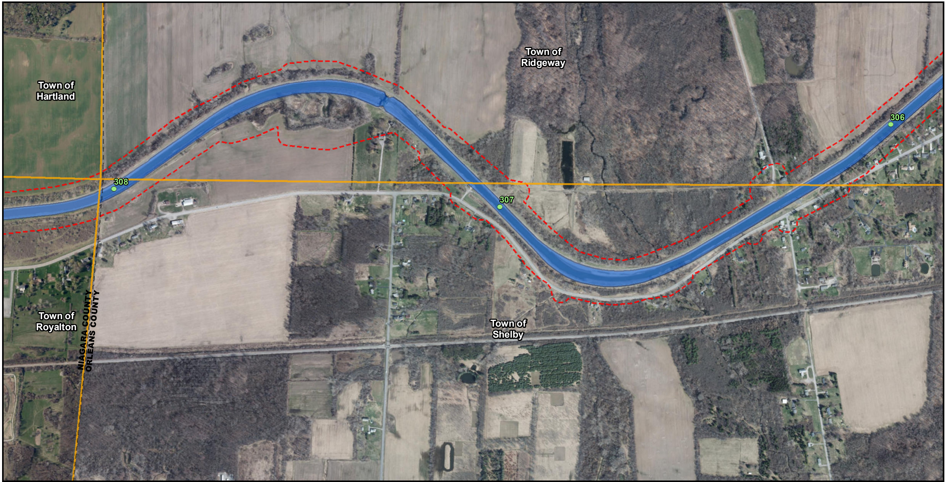
Figure 112F: Aquifers
